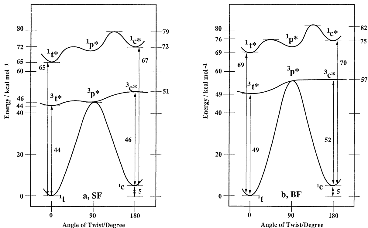
Fig. 4. Potential energy surfaces of cis-trans isomerization of SF (a) and BF (b).
